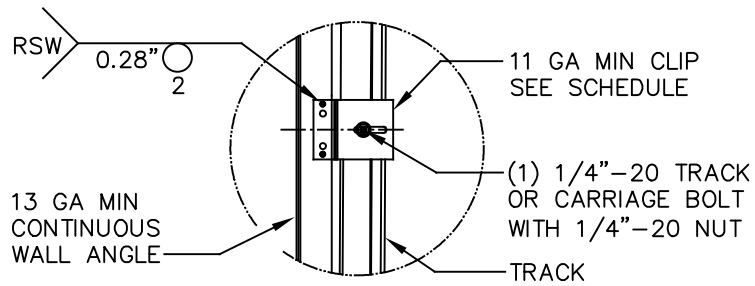
TYPICAL CLIP WELDING DETAIL
