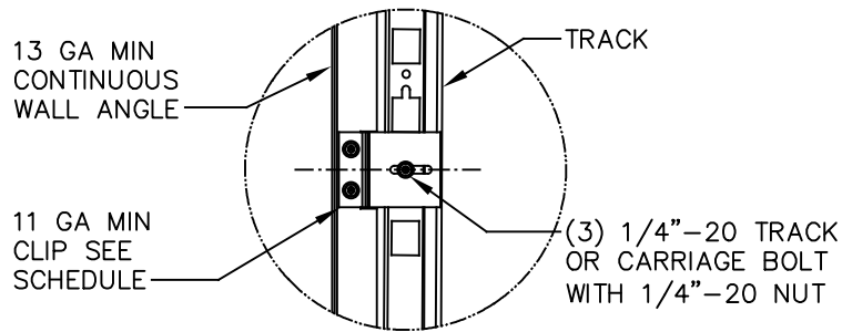
TYPICAL CLIP BOLTING DETAIL
