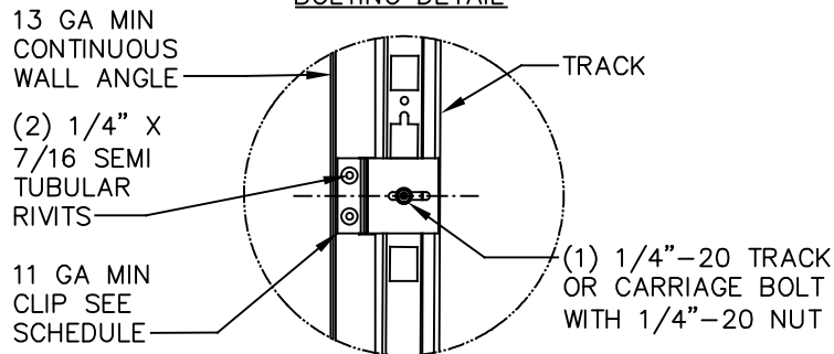
TYPICAL CLIP RIVETING DETAIL
